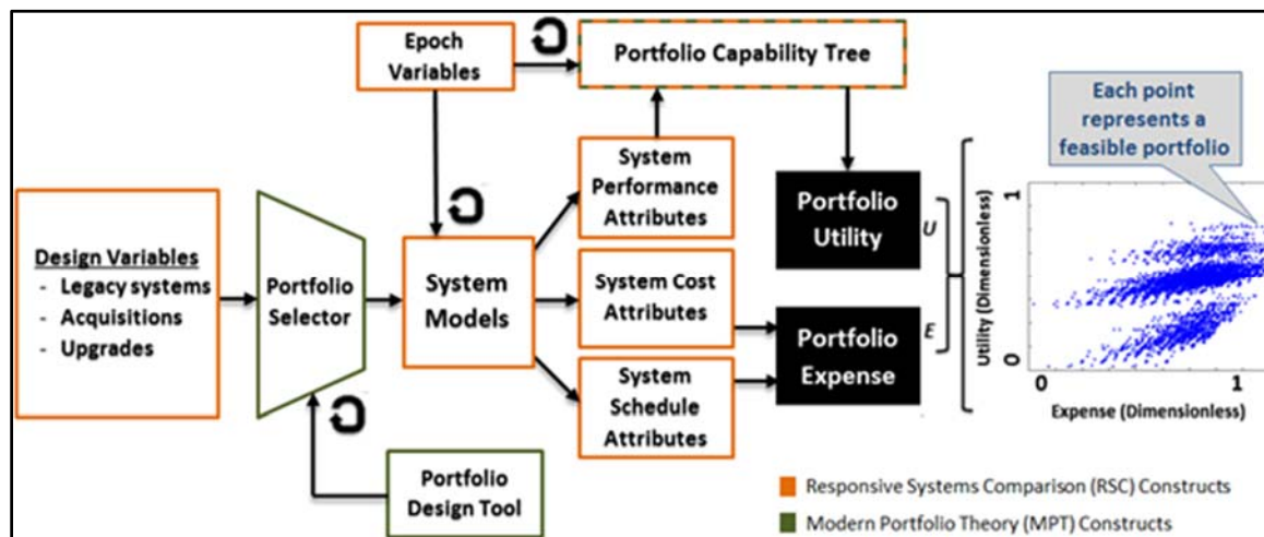
Figure 2. Portfolio-Level Epoch-Era Analysis for Affordability (PLEEAA) Process Model for Affordability Analysis
