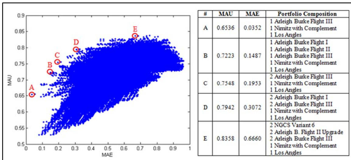
Figure 6. Portfolio Affordability Tradespace (MAU v. MAE) and Pareto Efficient Portfolios for the Baseline Epoch
