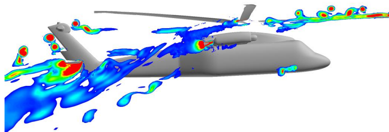
interactional aerodynamics
