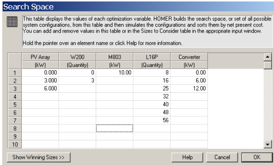
Figure 5. Search Space of a Unique Generator-PV-Wind System, with 242 Possible System Configurations (3 x 4 x 1 x 7 x 3 = 242)
