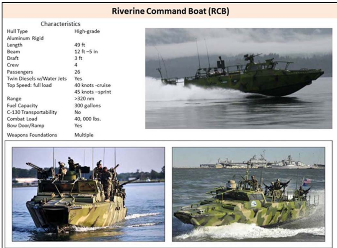
Figure 3. Riverine Command Boat (Thompson, 2011)
