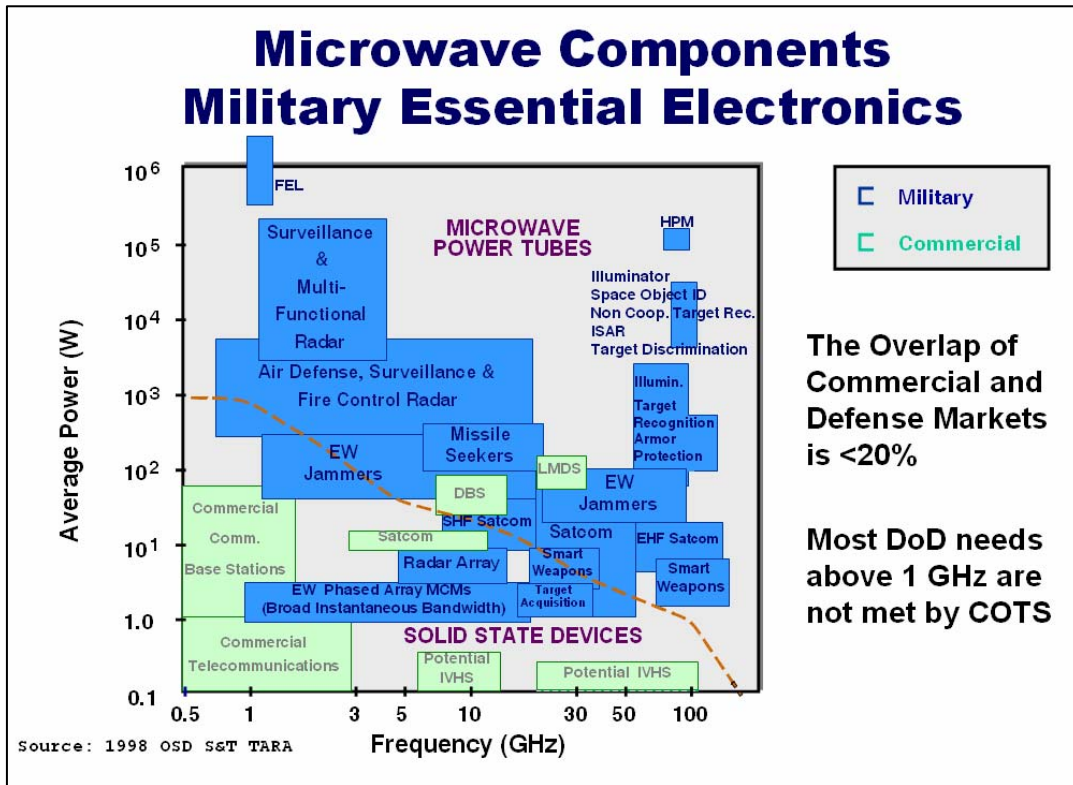
Figure 6. Microwave Components Military Essential Electronics Source: Dutkowski, E.J., Jr. (2004-2005)
