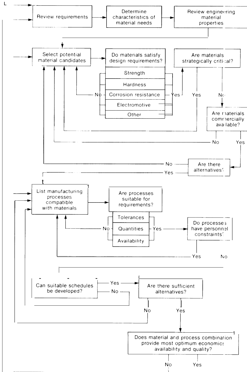
Figure 4-6-Decisions Concerning Producibility
