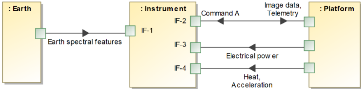
Figure 3. Example of Logical Capture of Interfaces
